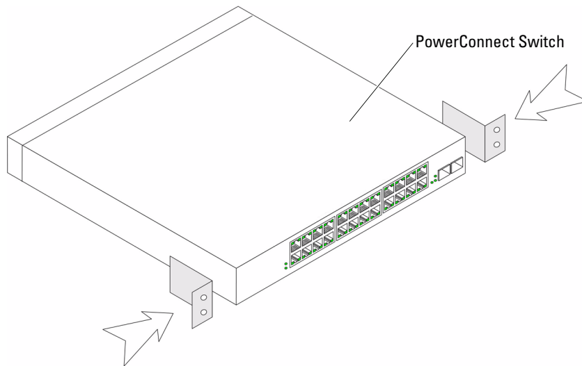
Figure 1-1. Bracket Installation for Rack Mounting
